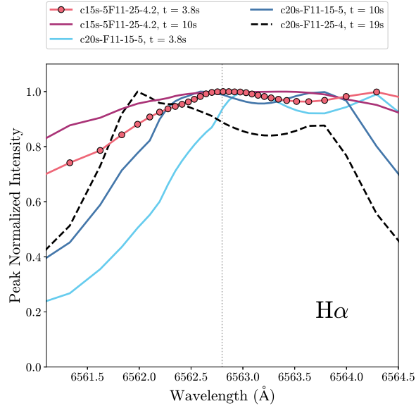
Figure 4. Representative H\alpha flare spectra from the three models in Table 1 normalized to the peak intensity. The wavelength range ( \Delta\lambda = 3.4 \text{ \AA} ) corresponds to a typical setup with the IBIS instrument on the Dunn Solar Telescope. In the near-blue wing, there are discernible differences in the slopes between the F11-15-5 (increasing to red side) and 5F11 (nearly flat across this limited wavelength range). The F11-25-4 model is shown at 19 s when the condensation begins to have an effect on the hydrogen line spectra (see Kuridze et al. 2015).
