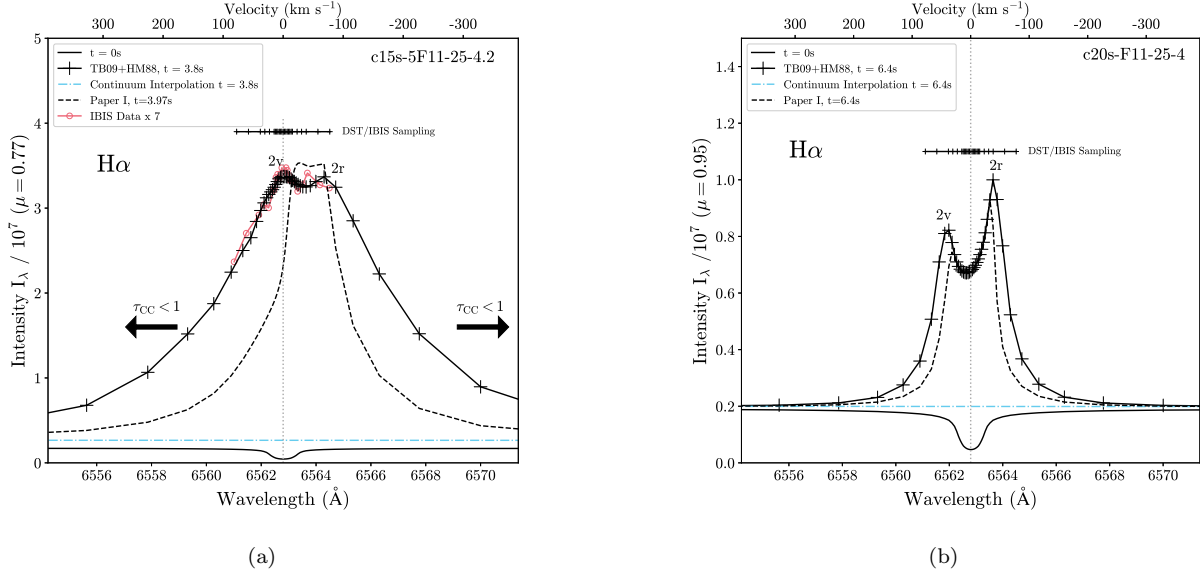
Figure 3. Model H\alpha flare spectra using the TB09+HM88 profiles in RADYN. These are improvements on recent works (dashed lines), which used the profiles corresponding to the broadening implementation of spectrum (4) in Figure 1(a). These two snapshots were chosen as the most similar in time to the snapshots that were analyzed in Figure 8 of Paper I (panel (a) here) and in Figure 7 in Kuridze et al. (2015) (panel (b) here). In this figure, the same viewing angles ( \mu ) are presented as in these two previous works. The flare continuum emergent intensity is interpolated across the line to demonstrate that in the higher beam flux model, the wings of the H\alpha line extend beyond this wavelength range ( \Delta\lambda = 17.15 \text{ \AA} , chosen as a representative wavelength range of a DKIST/ViSP window). The arrows in the left panel indicate the wavelengths at which the chromospheric condensation becomes optically thin over the TB09+HM88 spectrum (see text).
