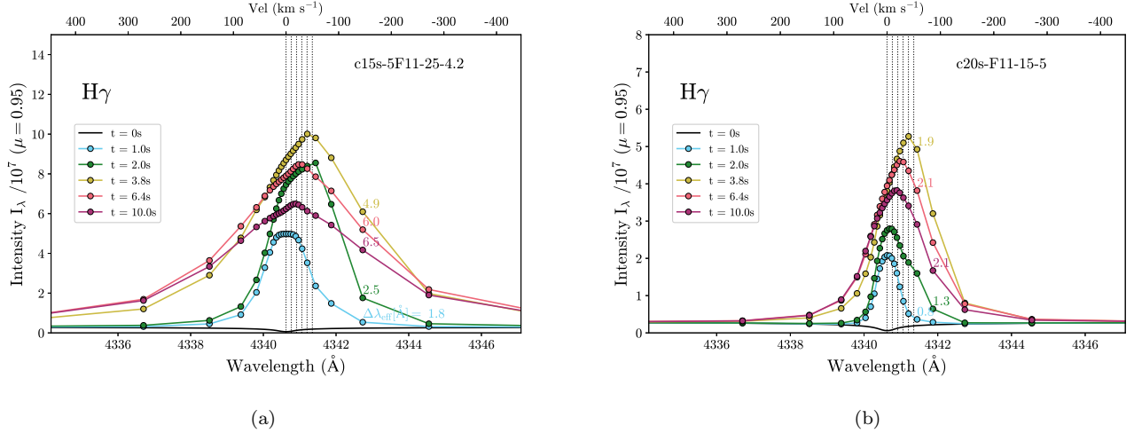
Figure 5. Time evolution of H \gamma for a wavelength window ( \Delta\lambda = 12.9 \text{ \AA} ) that is possible with a blue arm of the DKIST/ViSP. The profiles are shown at the same times for the 5F11 model (a) from Paper I and the F11 model (b) from Graham et al. (2020) . Vertical dashed lines indicate velocity shifts from 0 to -50 \text{ km s}^{-1} in increments of -10 \text{ km s}^{-1} , where negative velocities correspond to redshifts in the spectra and downflows in the hydrodynamics. The spectra are labeled by their calculated effective widths (see text). Note the different intensity scales for these two figures.
