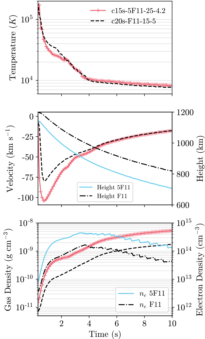
Figure 2. Evolution ( \Delta t = 0.1 s) of the atmospheric variables at the location of maximum gas density in the chromospheric condensation in the 5F11-25-4.2 and F11-15-5 models. The time range is shown for t = 0.3 - 10 s. The maximum gas density in the condensation ( \rho_{\max} ) is shown in the bottom panel (left axis). The locations of maximum densities in the respective condensations are shown in the middle panel, right axis.
