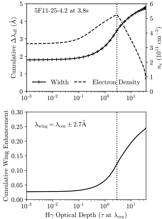
Figure 7. (Top) The curve-of-growth of the effective width of H \gamma through the chromospheric condensation at t = 3.8 s in the 5F11 model. The physical depth range in this figure is \Delta z \approx 30 km. At larger optical depths than at the maximum of n_e (vertical dotted line), the widths of the line increase further until reaching values near 4.9 \text{ \AA} in the emergent intensity spectrum. (Bottom) The cumulative of the contribution function at \lambda_{\text{cen}} \pm 2.7 \text{ \AA} relative to the cumulative of the contribution function at \lambda_{\text{cen}} . This closely follows the cumulative variation in effective width in the top panel.
